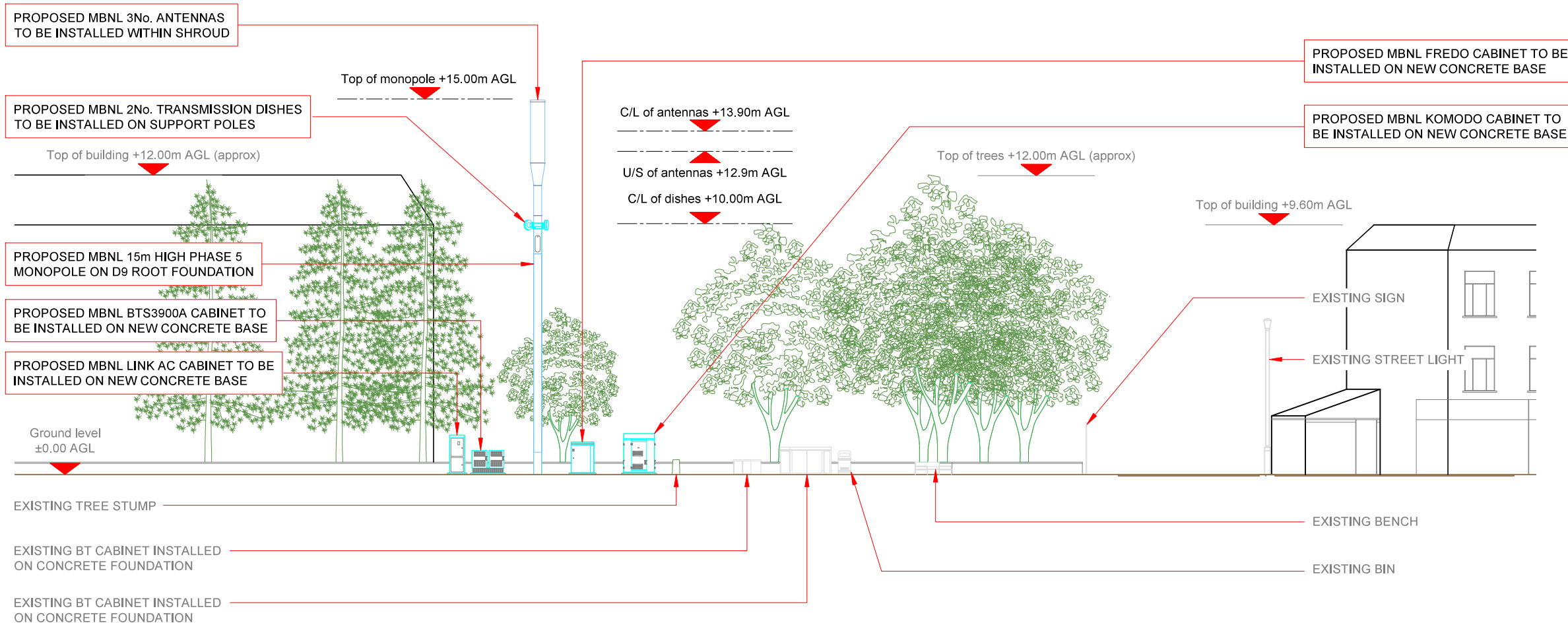
PROPOSED SHARED SITE ELEVATION
