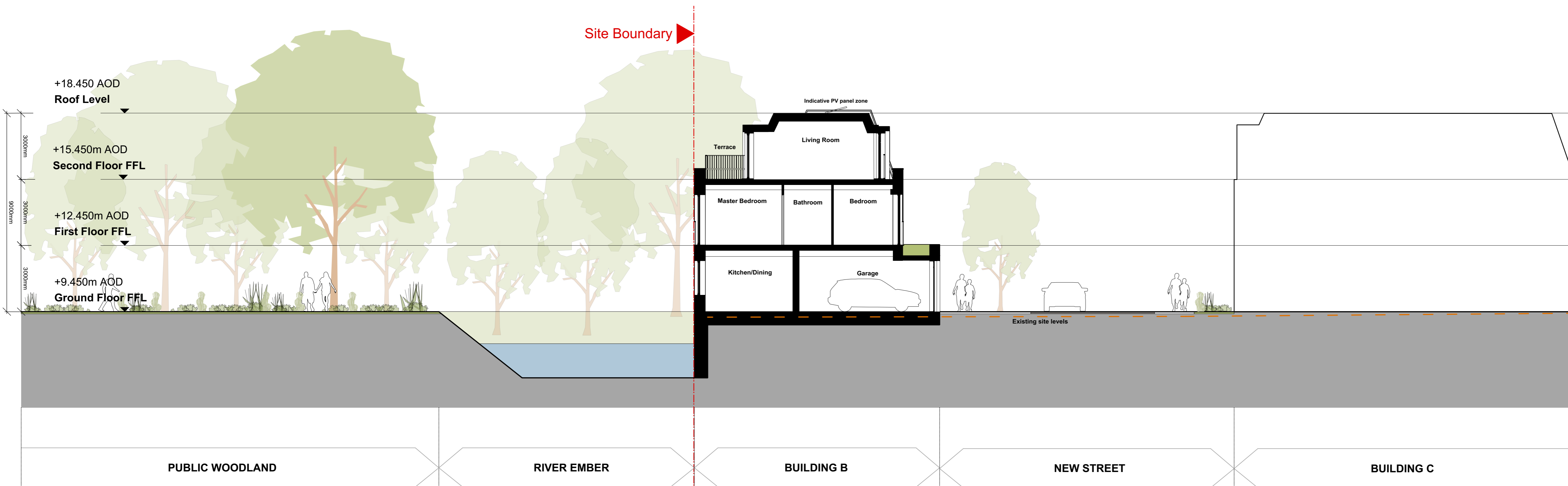
1 Building B Section AA Scale: 1:100
