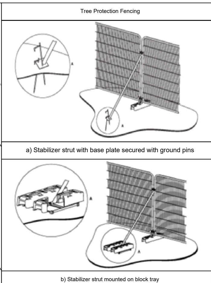
Images taken from British Standard BS27:2012 - Trees in relation to design, demolition and construction - Recommendations
